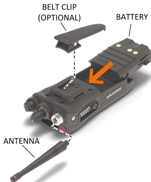
Figure 4-1: Radio Assembly
