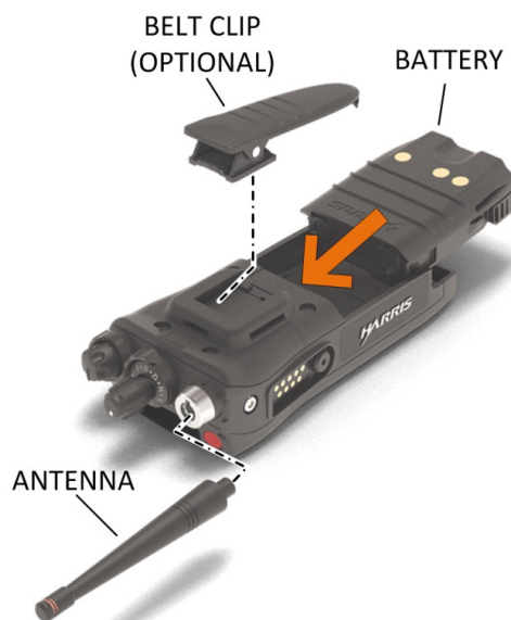
Figure 4-1: Radio Assembly
